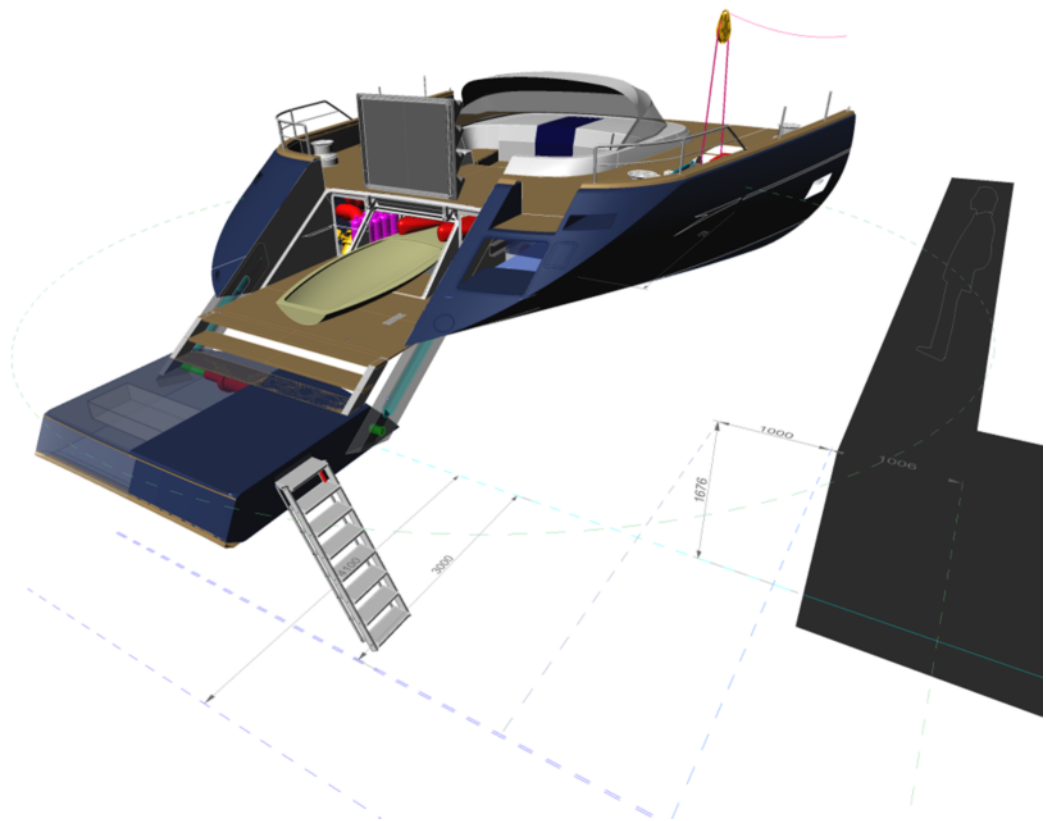
SY Twizzle stern platform 9 - HYDRAULIC SWIM LADDER DOWN.png
