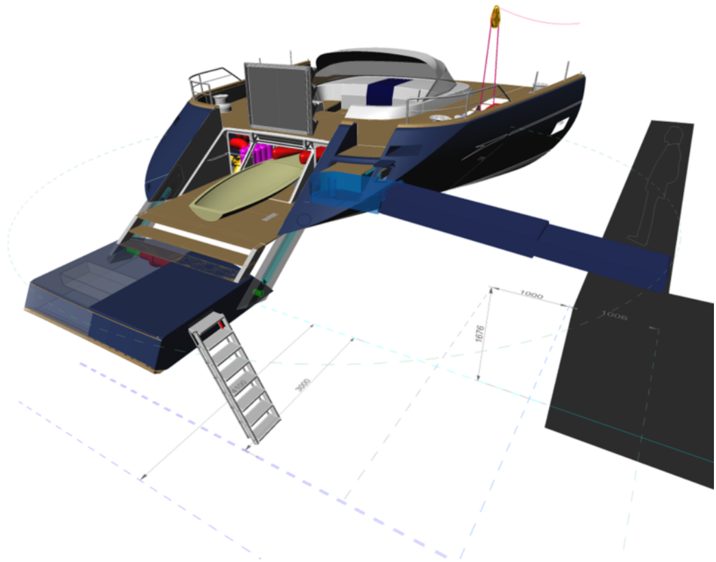
SY Twizzle stern platform 11 - PASSARELLE STB SWING.png
